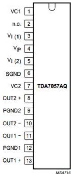
Pin configuration.
